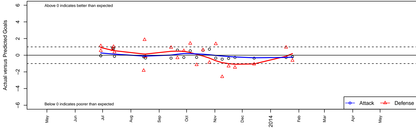
ISC Arsenal Red G01 Dots are actual minus expected GF (blue circles) and GA (red triangles). Blue line is smoothed change in attack strength. Red is smoothed change in defense strength.
